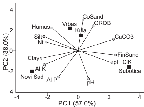
Figure 1: Principal components analysis of micro-abiotic soil parameters and Orobanchae intensity attack (OROB) following controlled inoculation in a greenhouse experiment.
