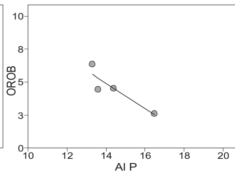
Figure 2: Linear correlation ( R^2=0.81 ; p=0.1006 ) between phosphorus availability (Al P=AL- P_2O_5 mg/100g) and Orobanchae intensity attack (OROB = weed plants/sunflower plant) following controlled inoculation of four soils
